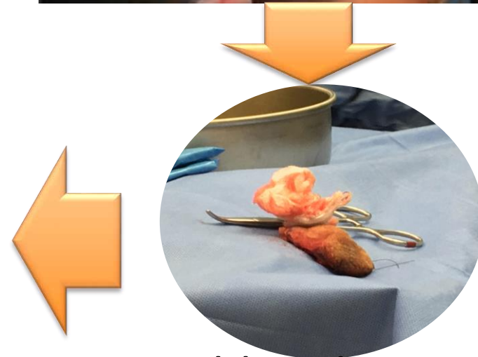
Ablated mass
